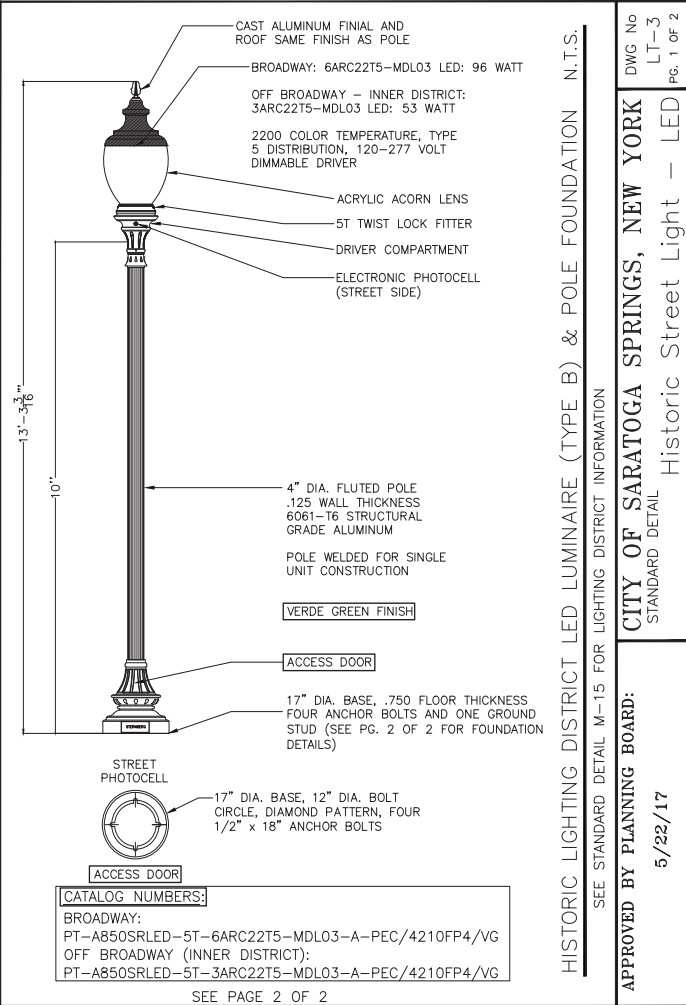
Current Saratoga Springs Standard Detail: Historic Street Light, LED version
